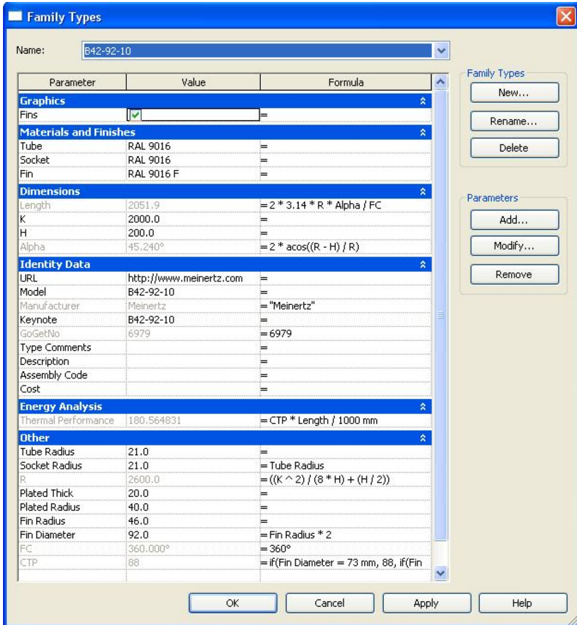
Figure A.02 Type B42-92-10 Family Parameter Reference
