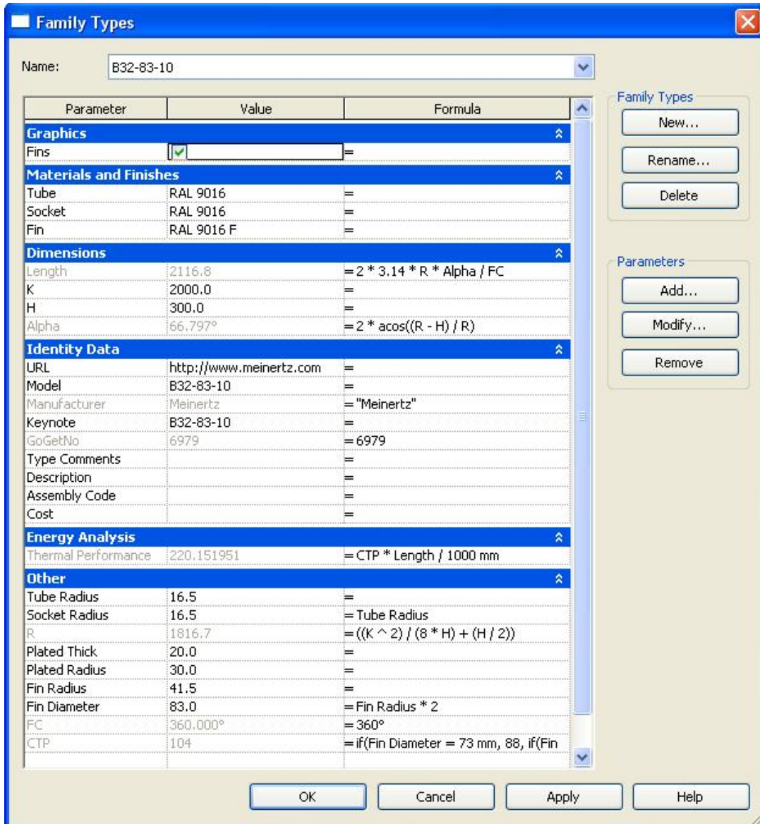
Figure A.01 Type B32-83-10 Family Parameter Reference
