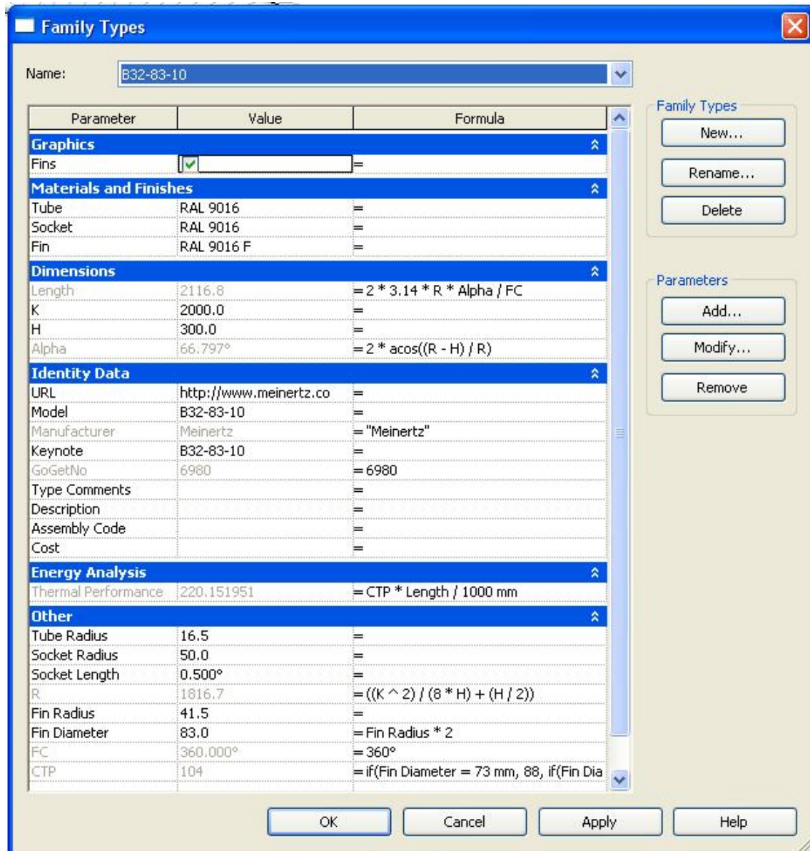
Figure A.01 Type B32-83-10 Family Parameter Reference
