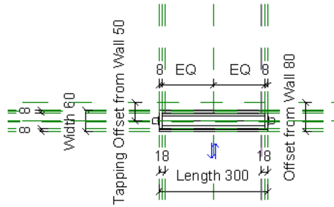
Main Family Plan Reference
