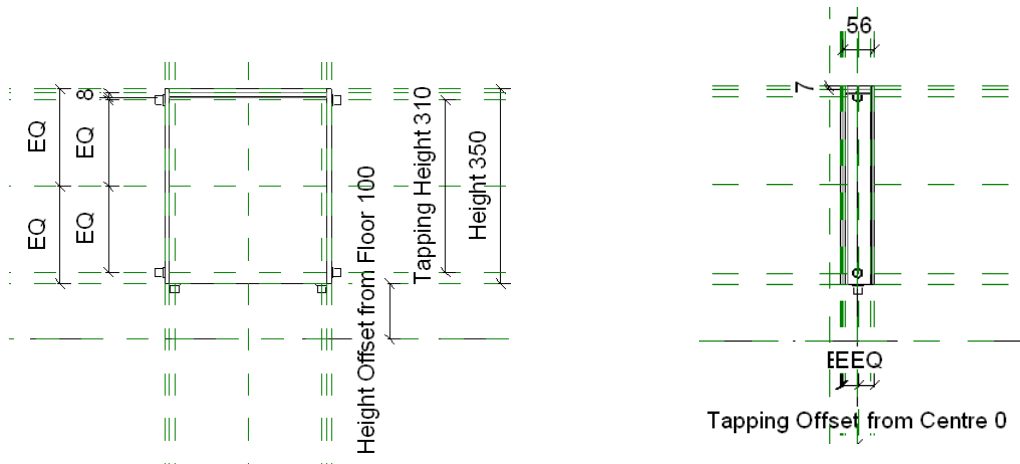
Main Family Side Elevation Reference
