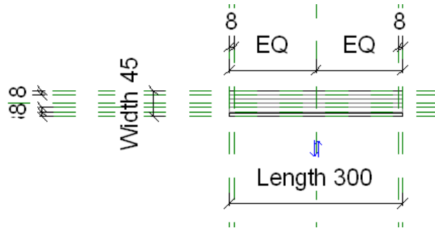
Main Family Plan Reference
