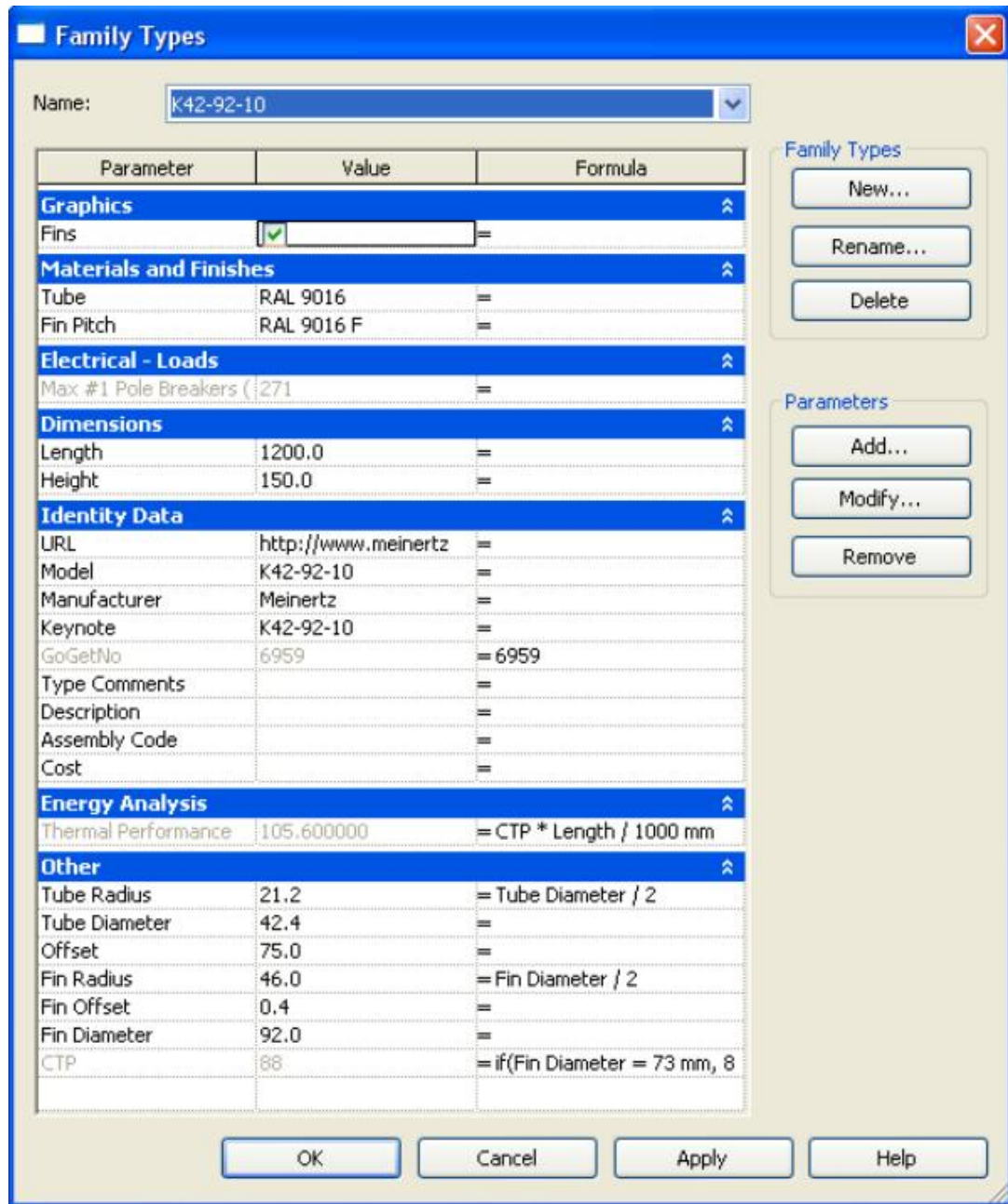
Figure A.04 Type - K42-92-10 Family Parameter Reference
