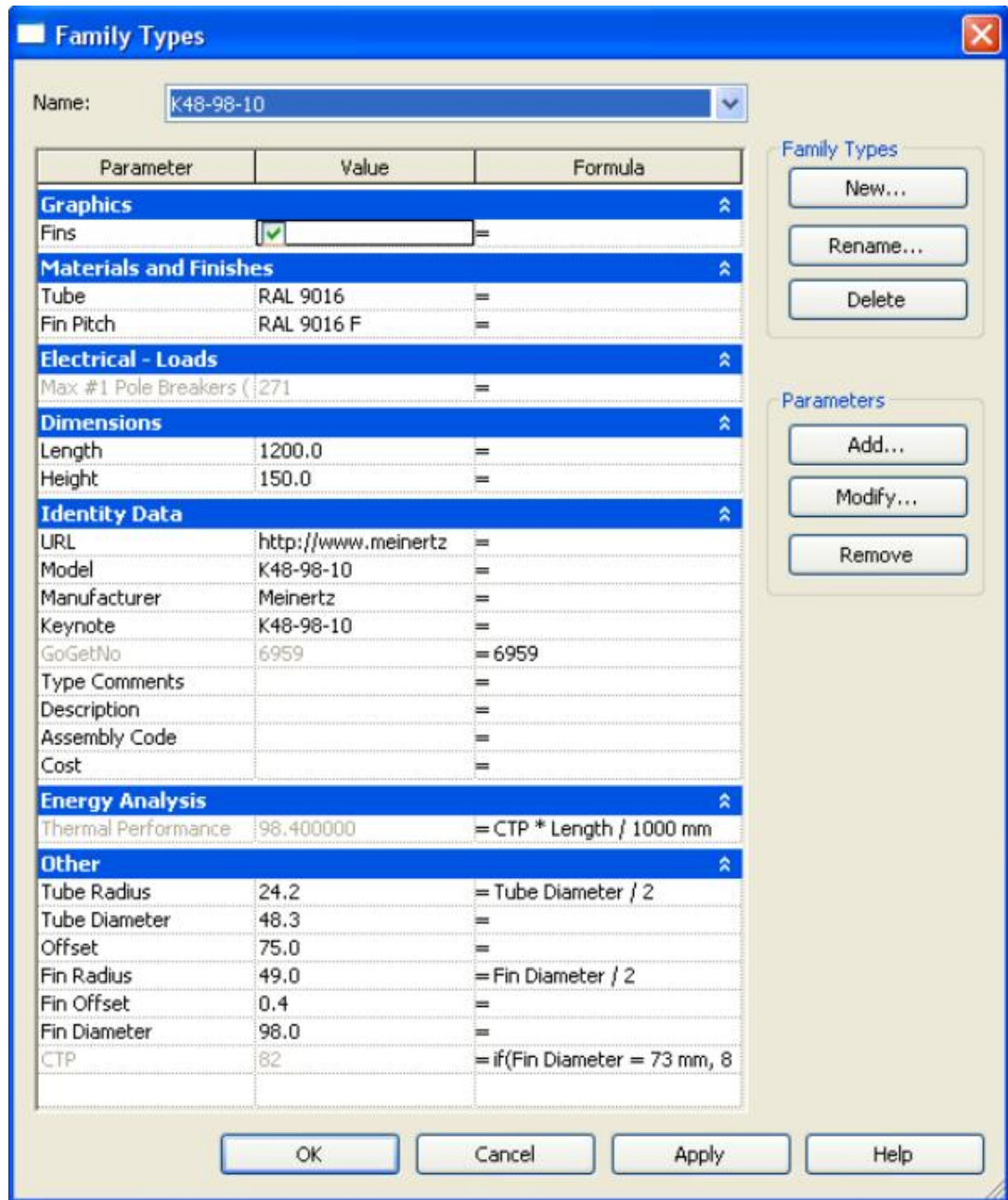
Figure A.05 Type - K48-98-10 Family Parameter Reference
