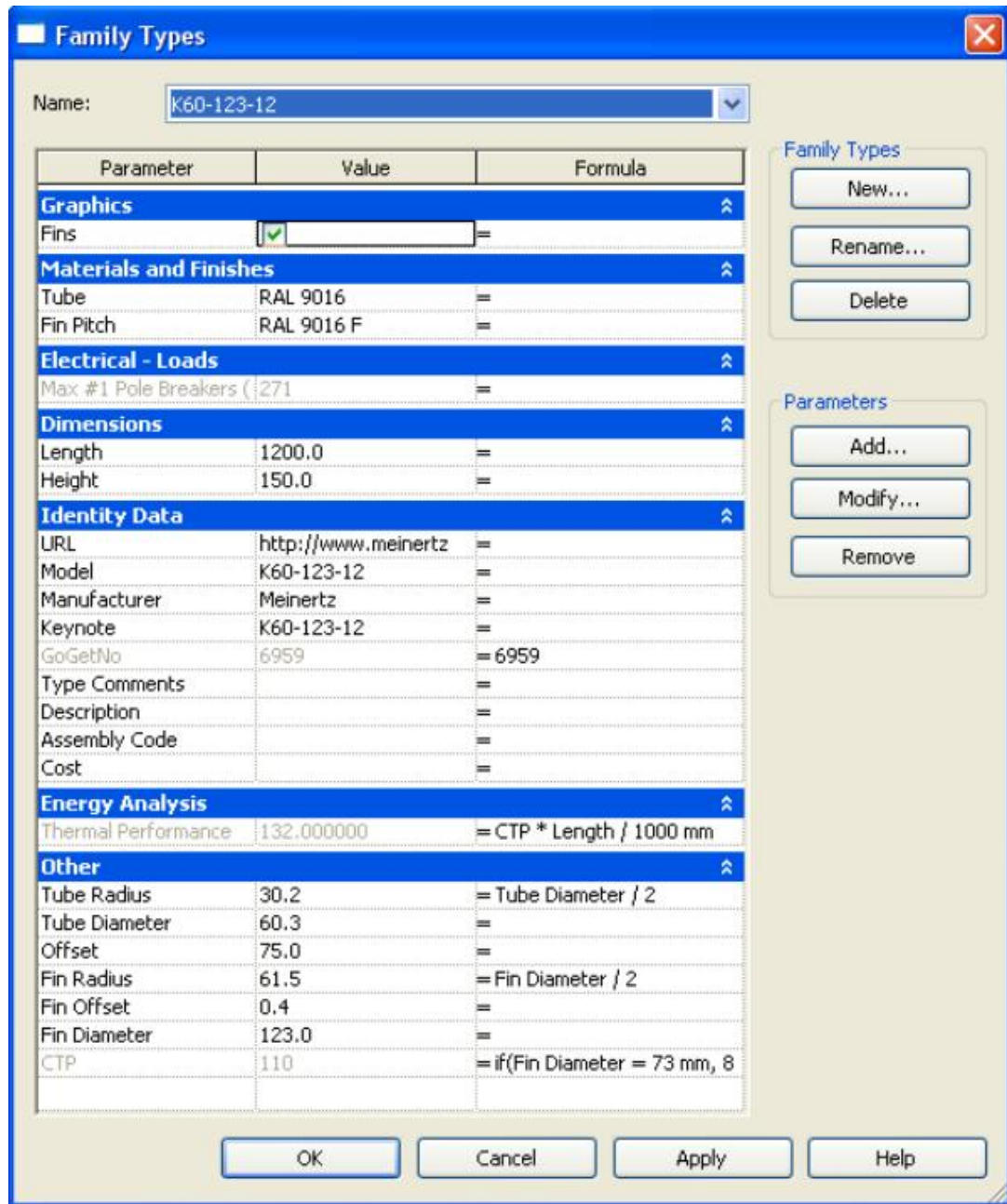
Figure A.07 Type - K60-123-12 Family Parameter Reference
