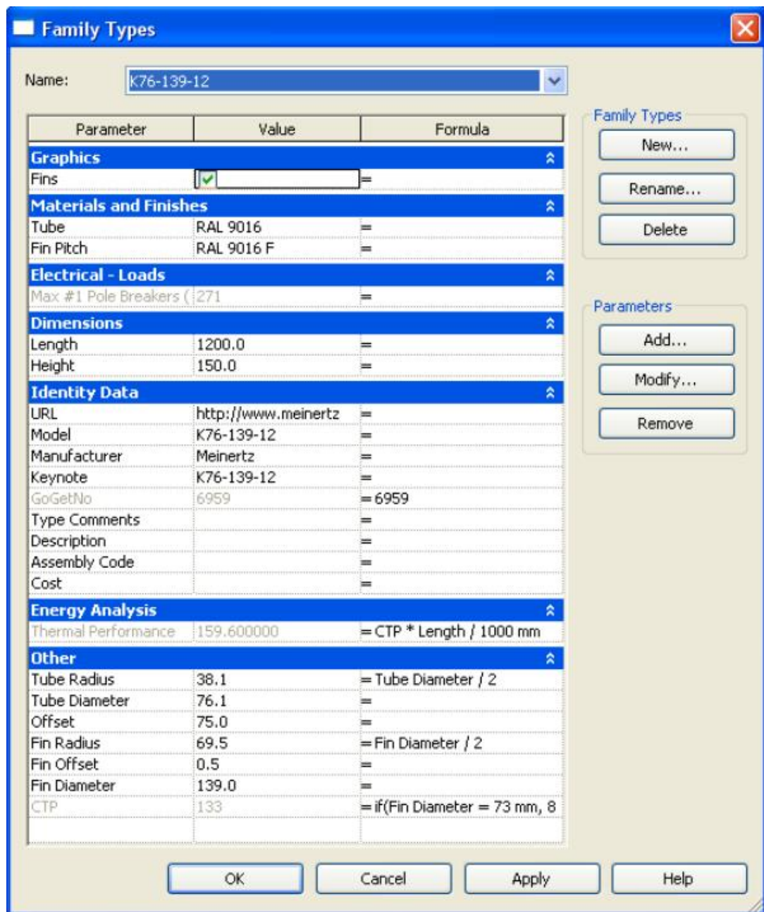
Figure A.08 Type - K76-139-12 Family Parameter Reference
