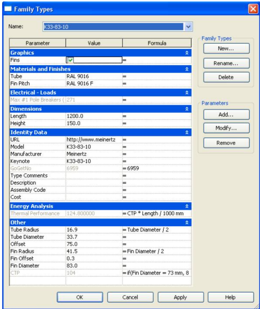
Figure A.03 Type - K33-83-10 Family Parameter Reference
