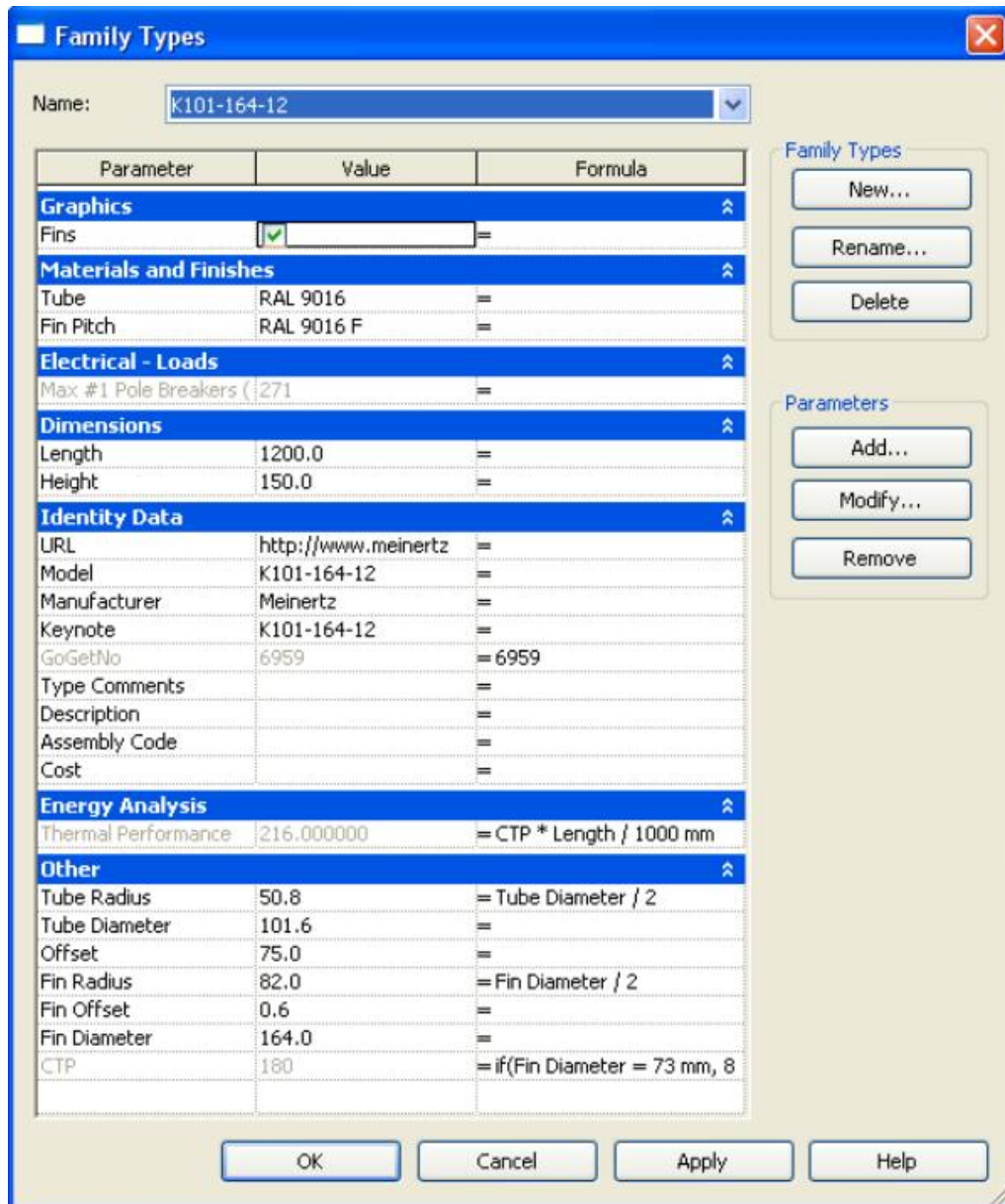
Figure A.01 Type - K101-164-12 Family Parameter Reference
