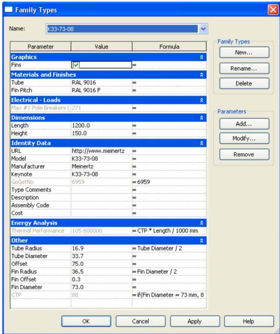
Figure A.02 Type - K33-73-08 Family Parameter Reference
