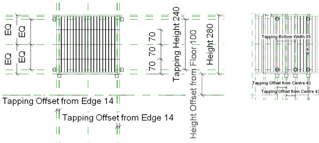
Main Family Side Elevation Reference
